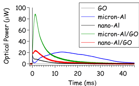
Figure 3-7: Emission from the laser-induced plasma (1 st sharp spike near time zero) and the subsequent combustion reactions of the GO, Al, and Al/GO particles ejected into the air above the sample surface.
