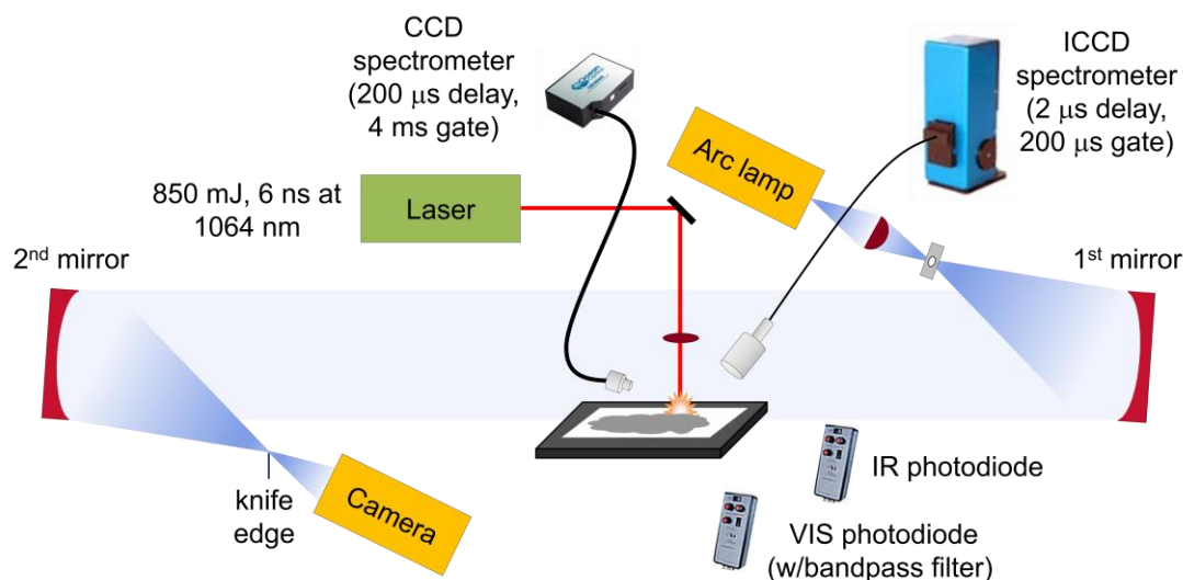
Figure 2-1: Experimental schematic for the laser ablation and excitation of Al/GO composites using LASEM. The emission from the laser-induced plasma and subsequent combustion reactions was detected with spectrometers gated to the appropriate time regime and time-resolved emission integrated over the visible (VIS) and infrared (IR) wavelengths was recorded with photodiodes. The laser-induced shock wave was recorded with a high-speed camera using schlieren imaging.
