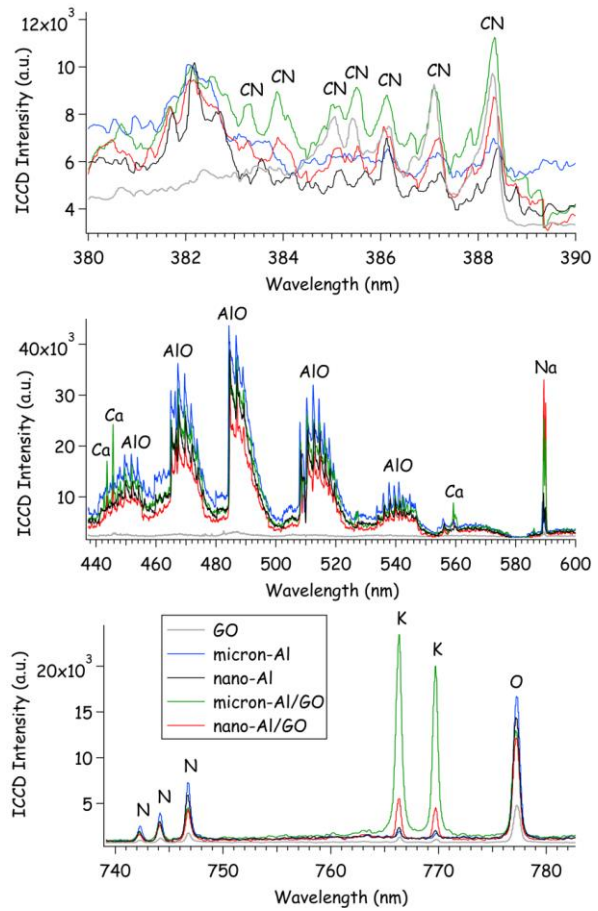
Figure 3-4: Emission spectra integrated over the first 200 \mu\text{s} of the laser-induced plasma lifetime (following a 2 \mu\text{s} delay to avoid the broadband continuum emission).
