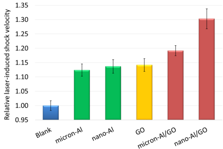
Figure 3-6: Relative laser-induced shock velocities for the blank tape substrate, micron-Al, nano-Al, GO, and the micron-Al/GO and nano-Al/GO composites.
