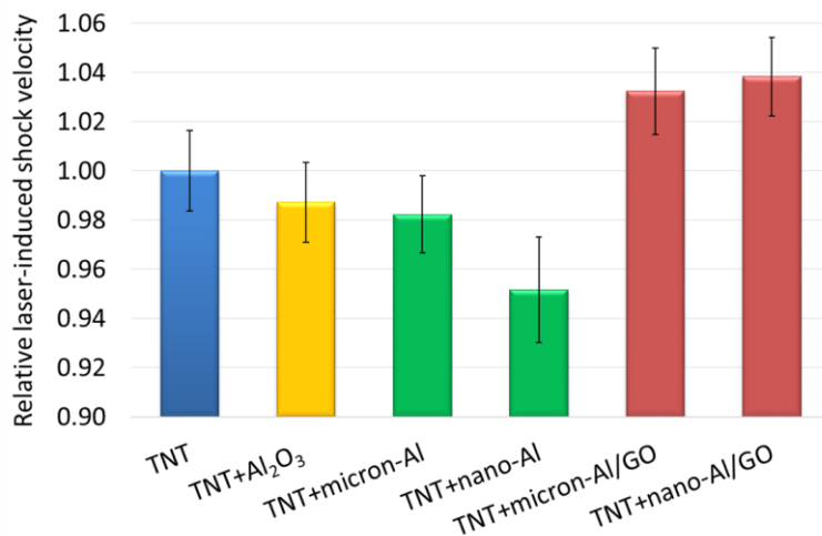
Figure 3-9: Relative laser-induced shock velocities for pure TNT, TNT+Al 2 O 3 , TNT+micron-Al, TNT+nano-Al, TNT+micron-Al/GO, and TNT+nano-Al/GO.
