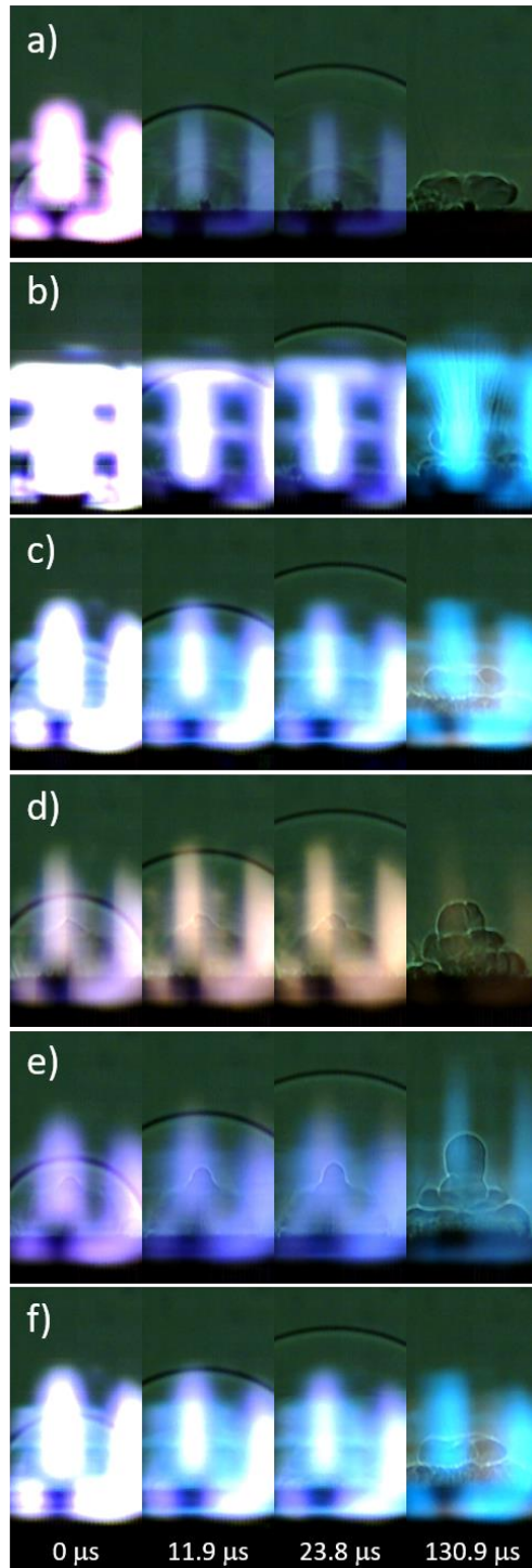
Figure 3-5: Snapshots from the high-speed video of laser-excited a) blank tape, b) micron-Al, c) nano-Al, d) GO, e) micron-Al/GO, and f) nano-Al/GO
