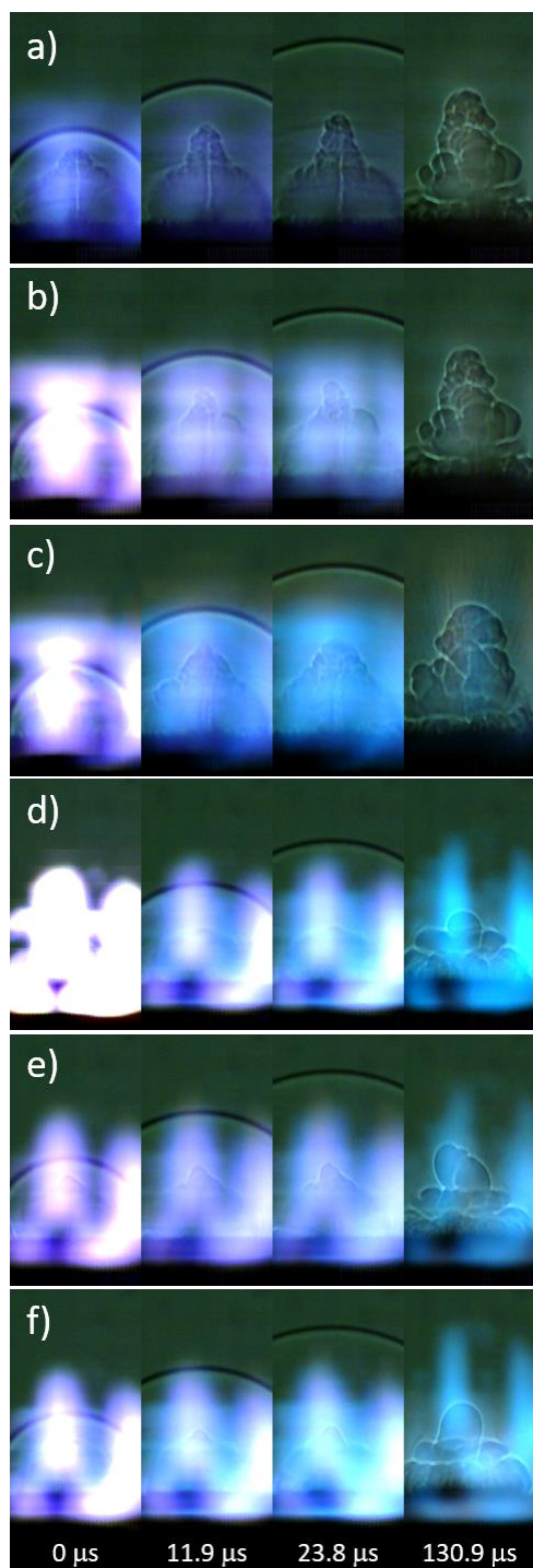
Figure 3-8: Snapshots from the high-speed video of laser-excited a) TNT, b) TNT+Al 2 O 3 , c) TNT+micron-Al, d) TNT+nano-Al, e) TNT+micron-Al/GO, and f) TNT+nano-Al/GO.
