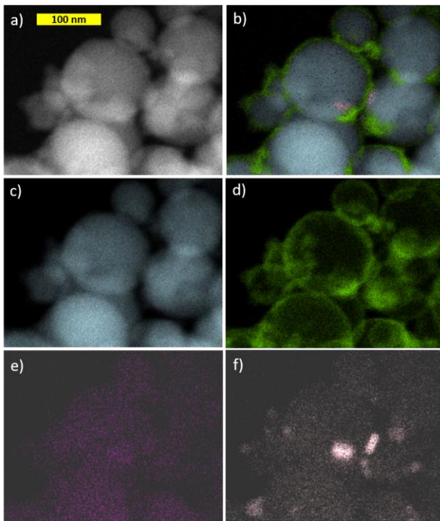
Figure 3-3: a) TEM image and b) the corresponding elemental map obtained using STEM showing the spatial distributions of c) aluminum, d) oxygen, e) carbon, and f) nitrogen in nano-Al/GO.
