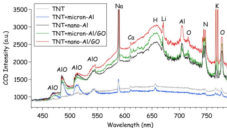
Figure 3-11: Emission spectra for TNT, TNT+Al, and TNT+Al/GO samples integrated over the first 4 ms of the combustion reactions following the laser-induced plasma.
