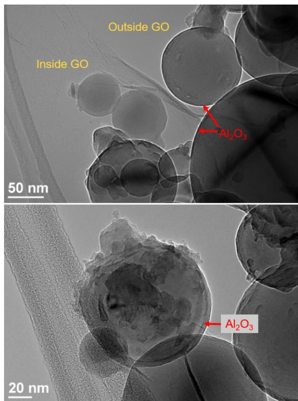
Figure 3-2: TEM images of nano-Al/GO showing the wrapping of the GO sheets around the nano-Al, the presence of the \text{Al}_2\text{O}_3 shell, and the contamination present on some of the Al particle surfaces.
