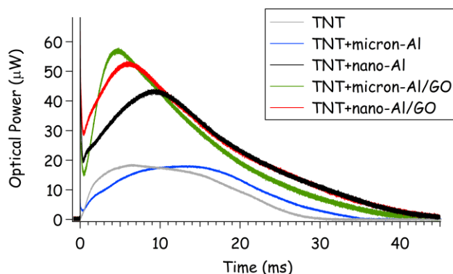
Figure 3-10: Emission from the laser-induced plasma (1 st sharp spike near time zero) and the subsequent combustion reactions of TNT, TNT+Al, and TNT+Al/GO particles ejected into the air above the sample surface.
